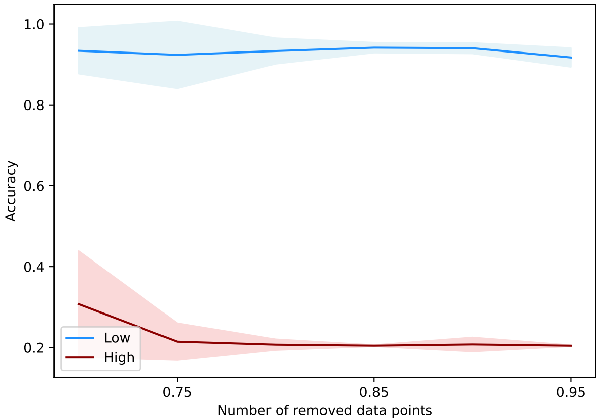
DataAttrOpt(10000, 0.1, 15, best, +b, alpha=best) - bbc-embeddings
